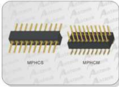
2.54mm Machined Pin Header
