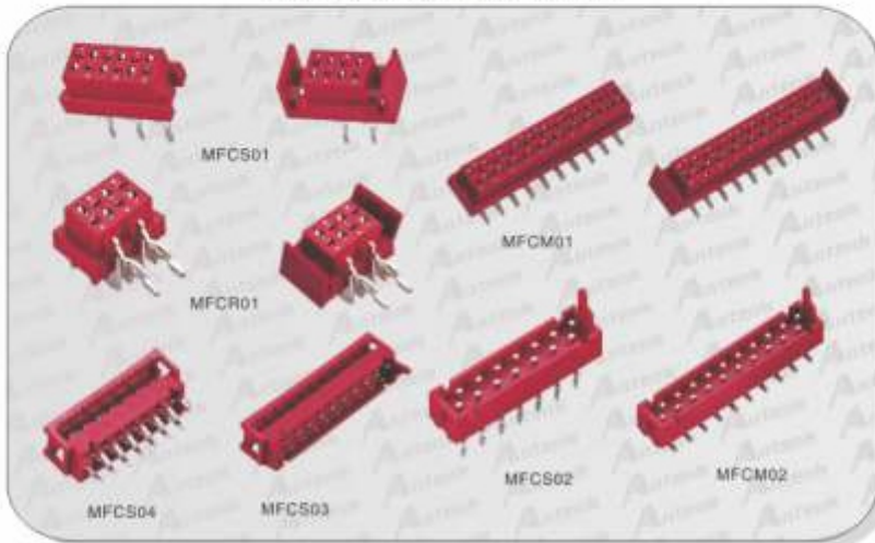
Micro Match Connectors Type
